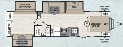
312 BHSLE ♦ Exterior Length 36' 9"
