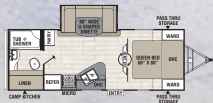
231 RBDS ♦ Exterior Length 26' 10"
