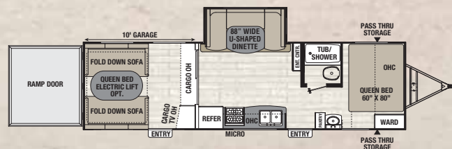
301 BLDS ♦ Exterior Length 33' 7"
