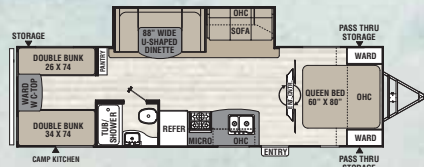
292 BHSLE ♦ Exterior Length 33' 5"
