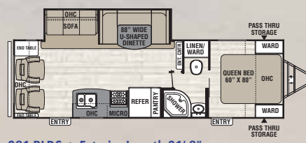
281 RLDS ♦ Exterior Length 31' 8"
