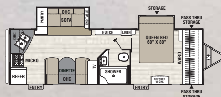
276 RKDS ♦ Exterior Length 31' 6"
