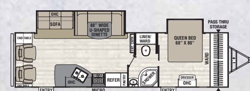
297 RLDS ♦ Exterior Length 35' 2"
