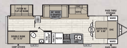
310 BHDS ♦ Exterior Length 35' 7"
