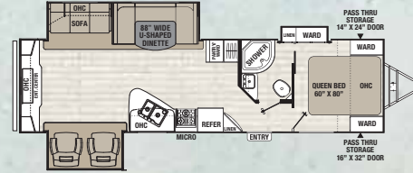
298 RLSLE ♦ Exterior Length 35' 2"
