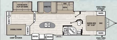
320 BHSLE ♦ Exterior Length 36' 11"
