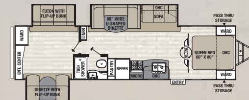
312 BHDS ♦ Exterior Length 36' 9"
