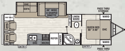
281 RLSLE ♦ Exterior Length 31' 8"
