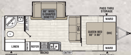
24 SE ♦ Exterior Length 28' 11"
